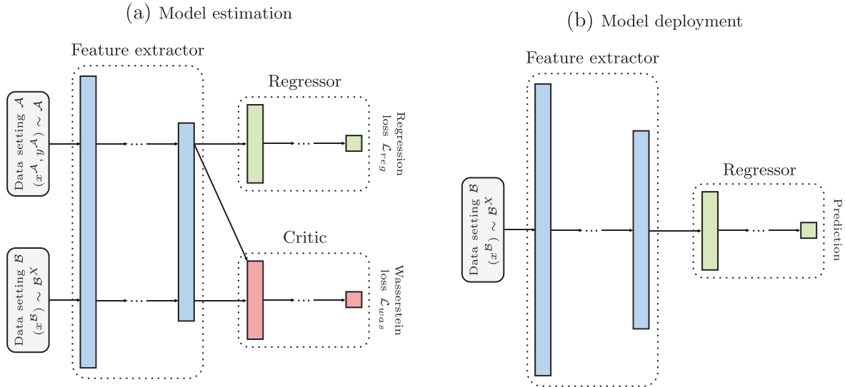
FIGURE 7 Model specification based on the feature extractor f_e , the regressor f_r , and the critic f_c . The use of the model depends on whether (a) parameters should be estimated or (b) predictions should be made upon deployment. [Color figure can be viewed at wileyonlinelibrary.com]
